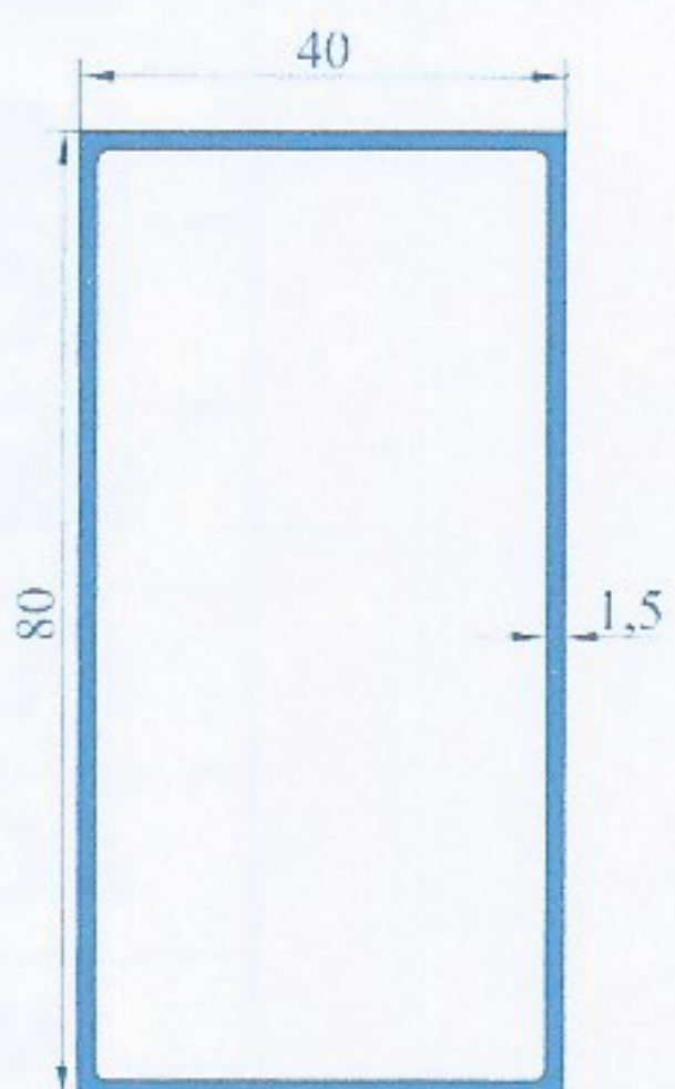
TUBO RECTANGULAR 80x40x1,5 mm.
