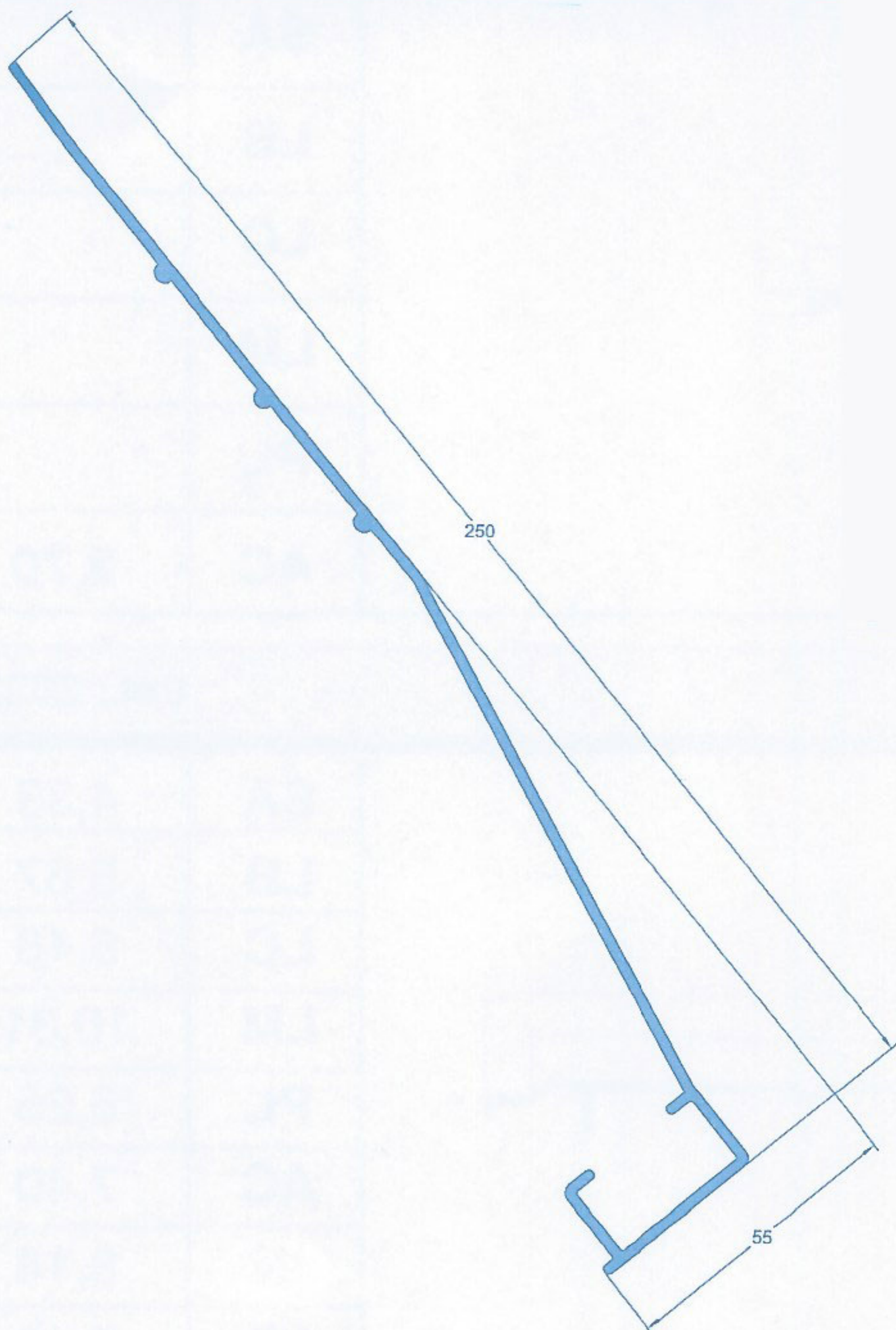
ALFEIZAR
